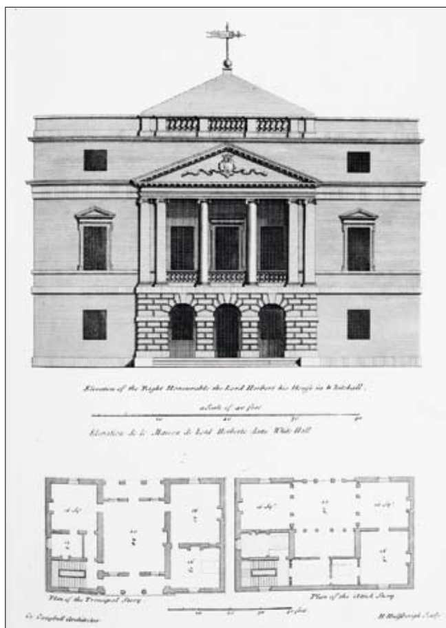
Obr. 8: C. Campbell, dům Lorda Herberta ve Whitehallu 1725 (repro z C. Campbell, Vitruvius Britannicus or The British Architect , 3. sv. London 1725, s. 48).
